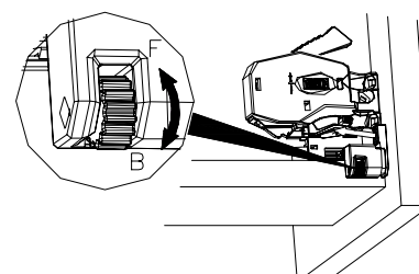
Depth regulation 0~+3 mm
