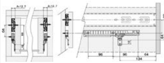
Soft-close damper installation for ball-bearing runners (A=12,7 mm)
