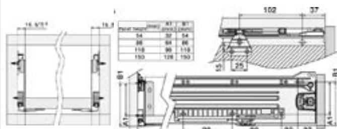
Soft-close damper installation for Metal Boxes
