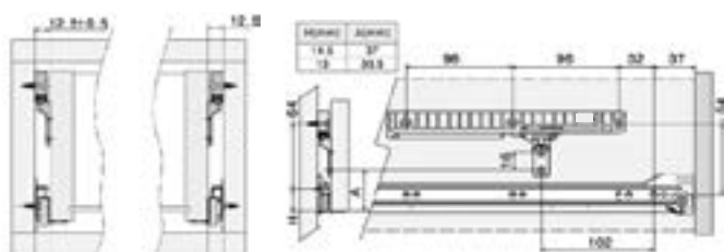
Soft-close damper installation for roller runners
